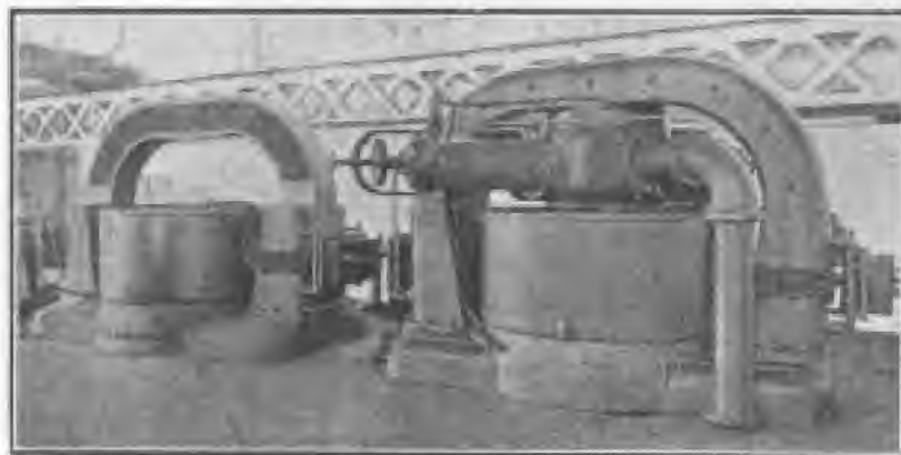
The Arc Converter of 50 Kilowatt 18 Capacity, at the Cavite Radio Station
